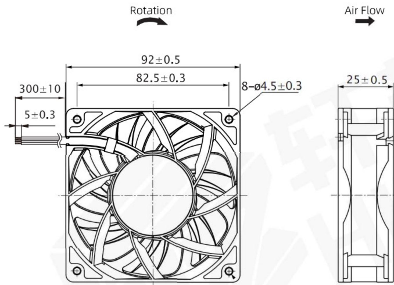
尺寸图Dimension Drawing (Unit : mm)
