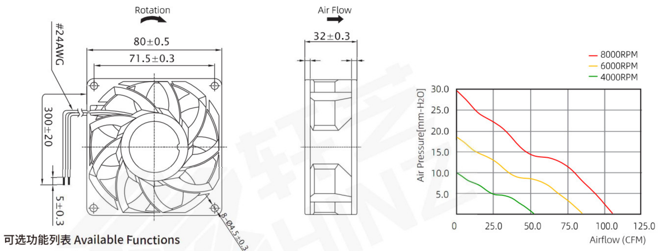
尺寸图Dimension Drawing (Unit : mm)
