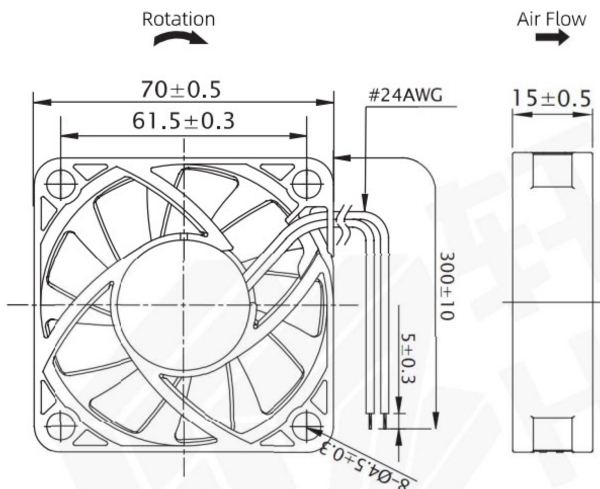
尺寸图Dimension Drawing (Unit : mm)
