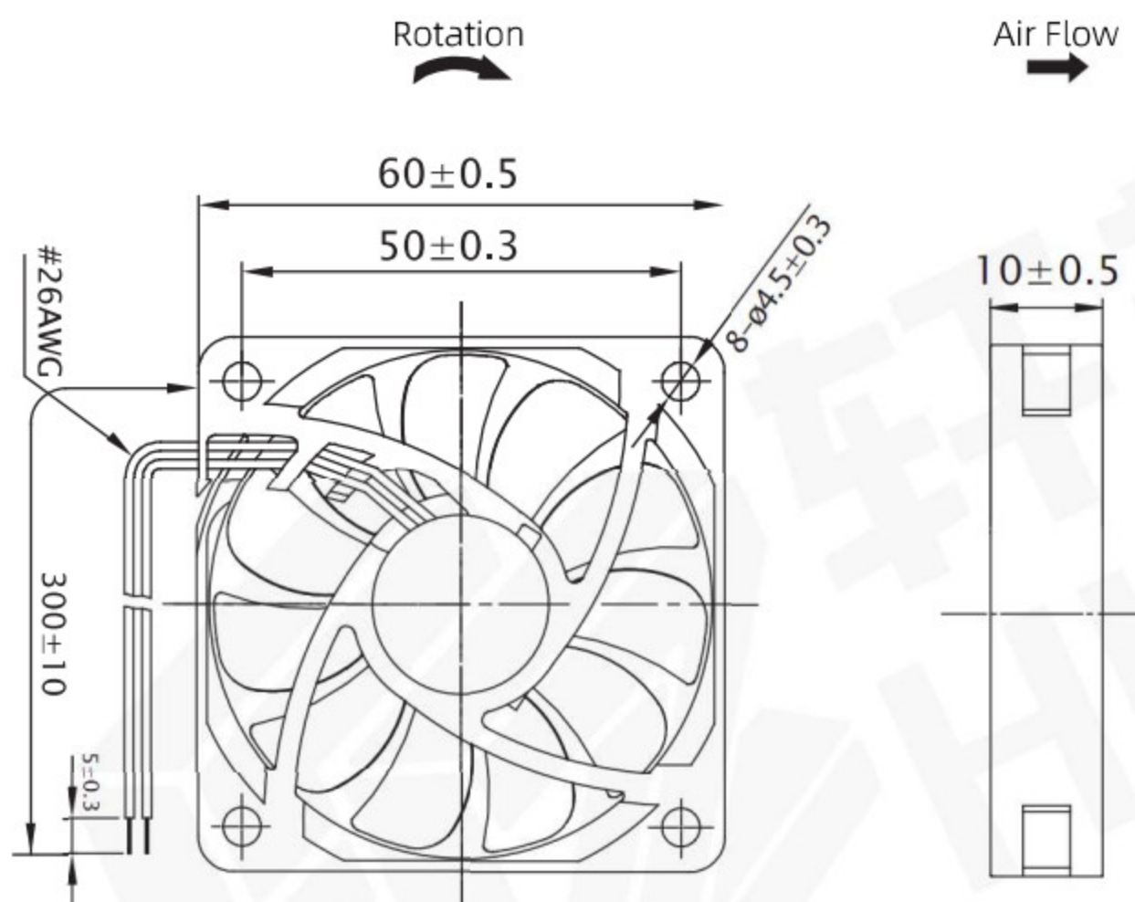
尺寸图Dimension Drawing (Unit : mm)
