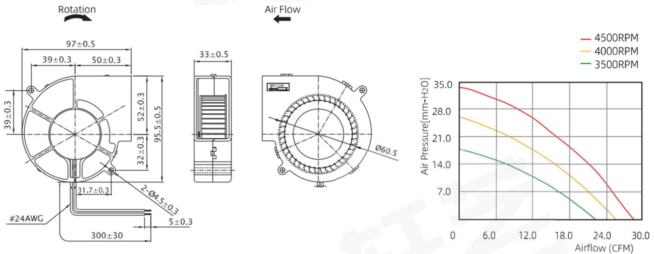
尺寸图Dimension Drawing (Unit : mm)
