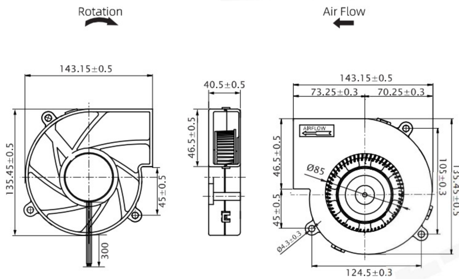
尺寸图Dimension Drawing (Unit : mm)
