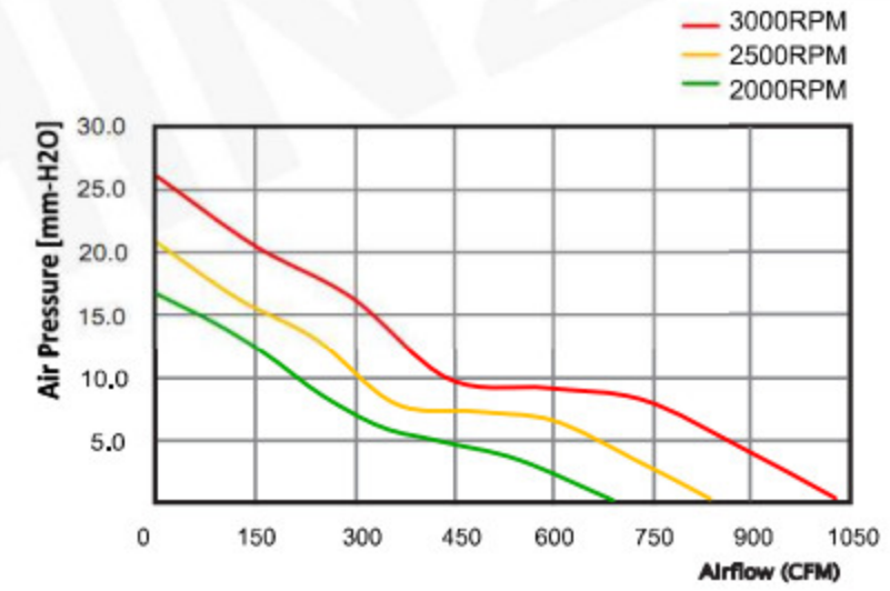
P-Q 曲线图/P-Q Curve Chart
