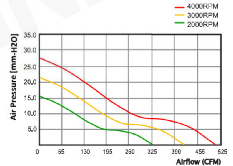
P-Q 曲线图/P-Q Curve Chart
