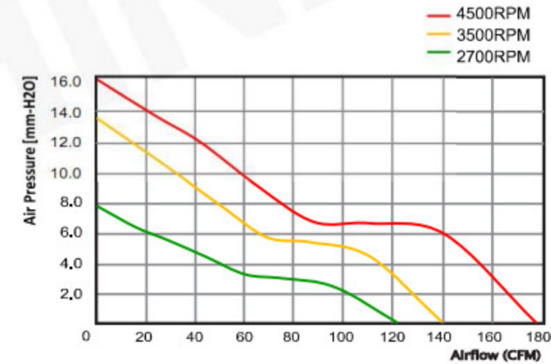
P-Q 曲线图/P-Q Curve Chart
