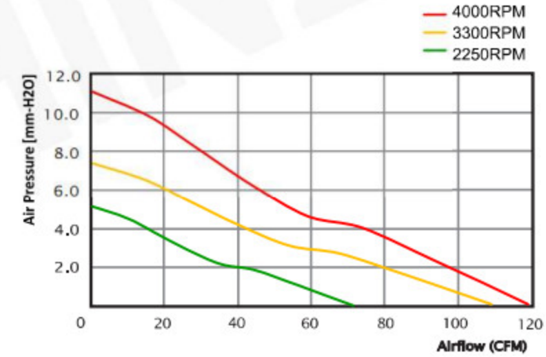
P-Q 曲线图/P-Q Curve Chart
