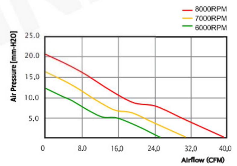
P-Q 曲线图/P-Q Curve Chart
