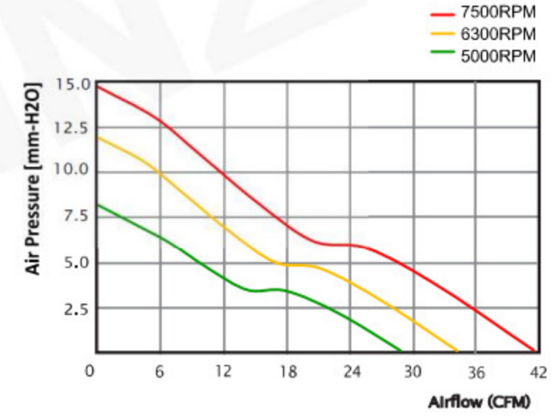
P-Q 曲线图/P-Q Curve Chart
