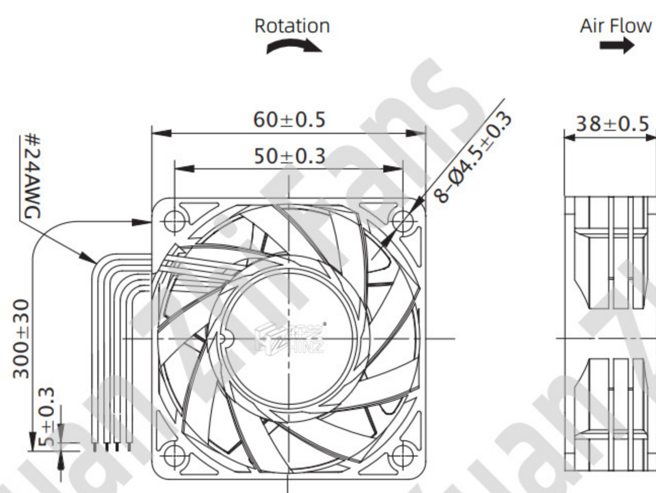
尺寸图Dimension Drawing (Unit : mm)
