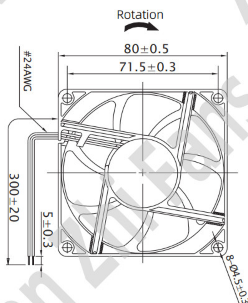
尺寸图Dimension Drawing (Unit : mm)
