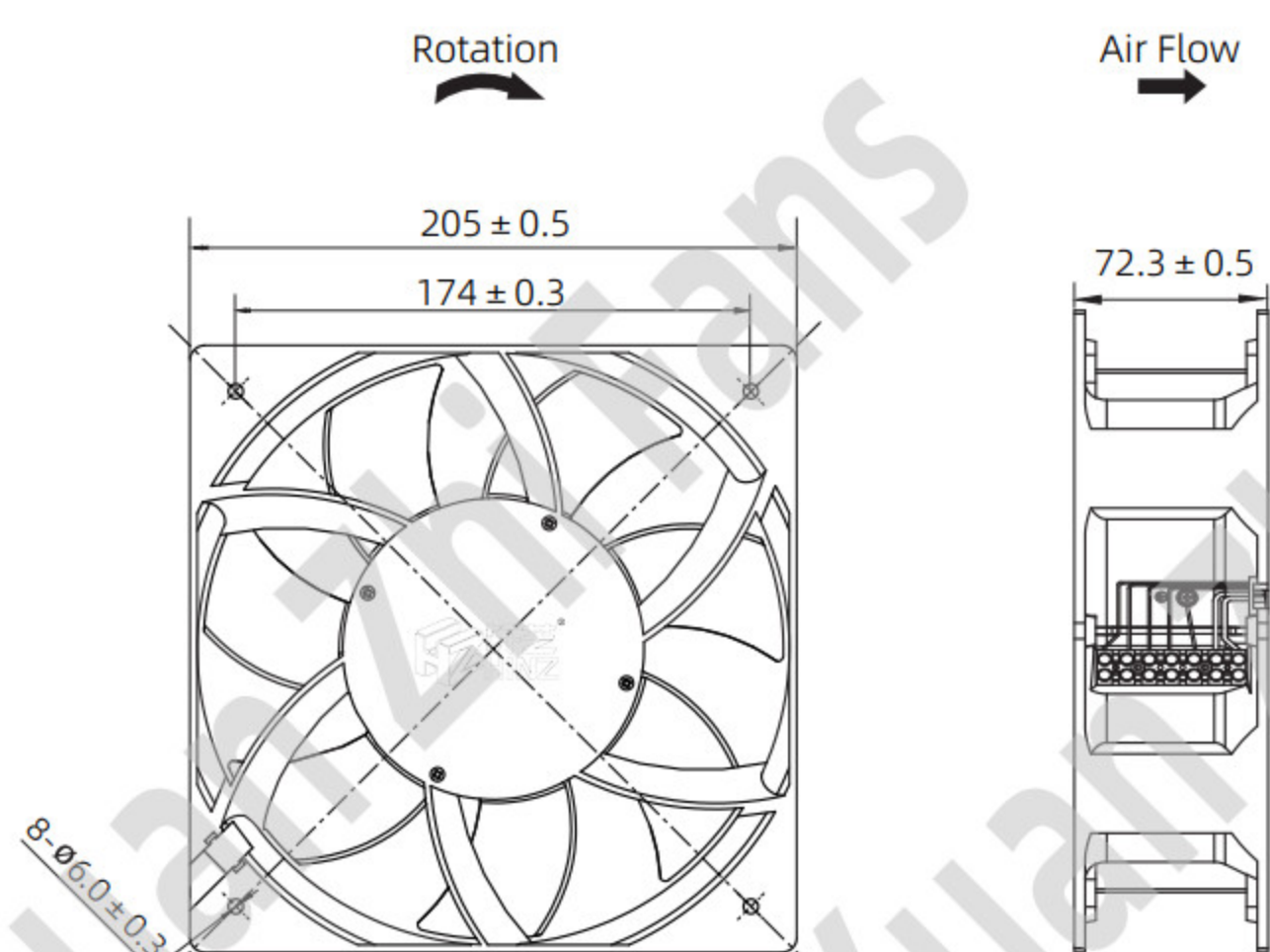
尺寸图Dimension Drawing (Unit : mm)
