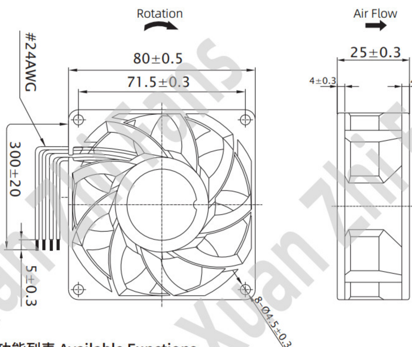
尺寸图Dimension Drawing (Unit : mm)
