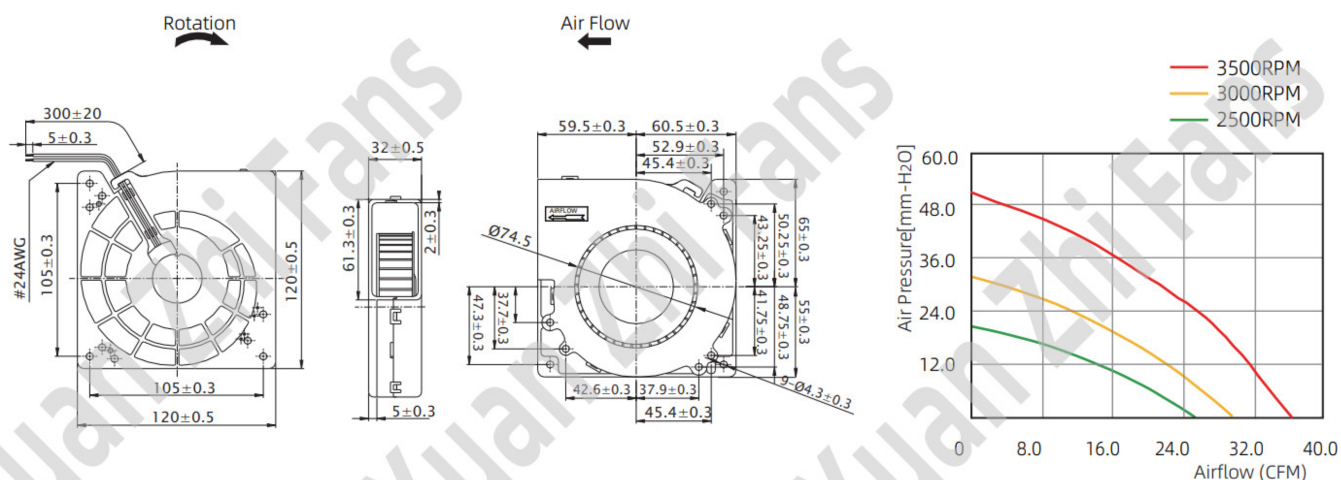
尺寸图Dimension Drawing (Unit : mm)
