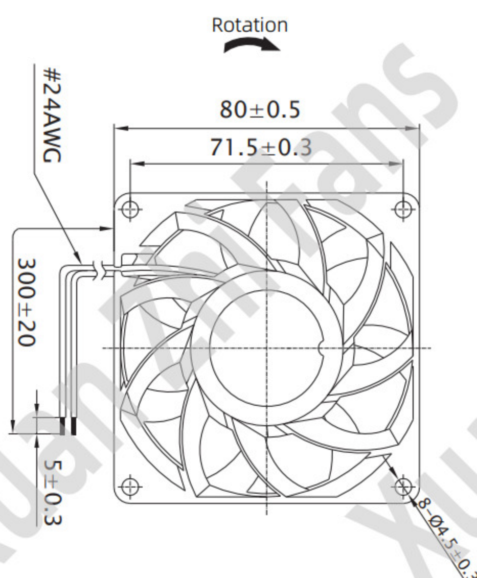
尺寸图Dimension Drawing (Unit : mm)
