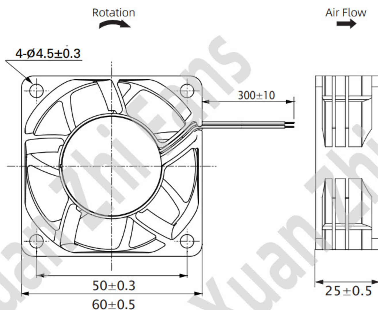
尺寸图Dimension Drawing (Unit : mm)
