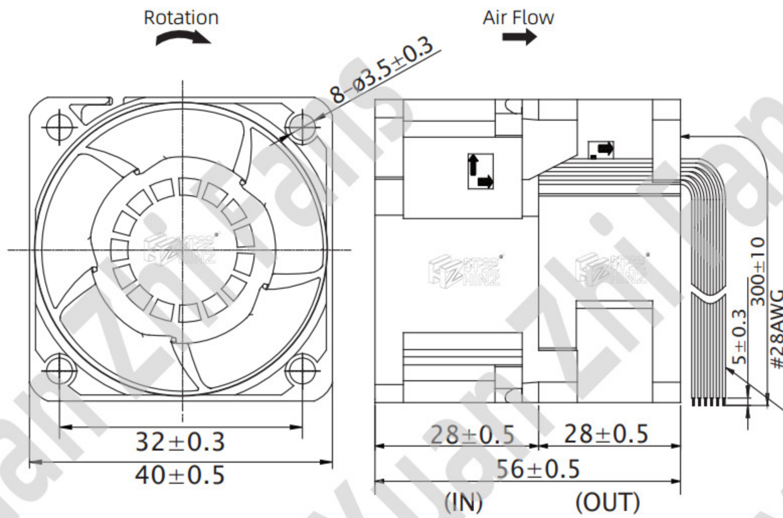
尺寸图Dimension Drawing (Unit : mm)
