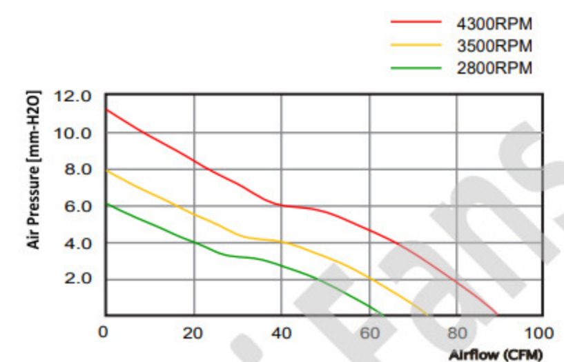
P-Q 曲线图/P-Q Curve Chart
