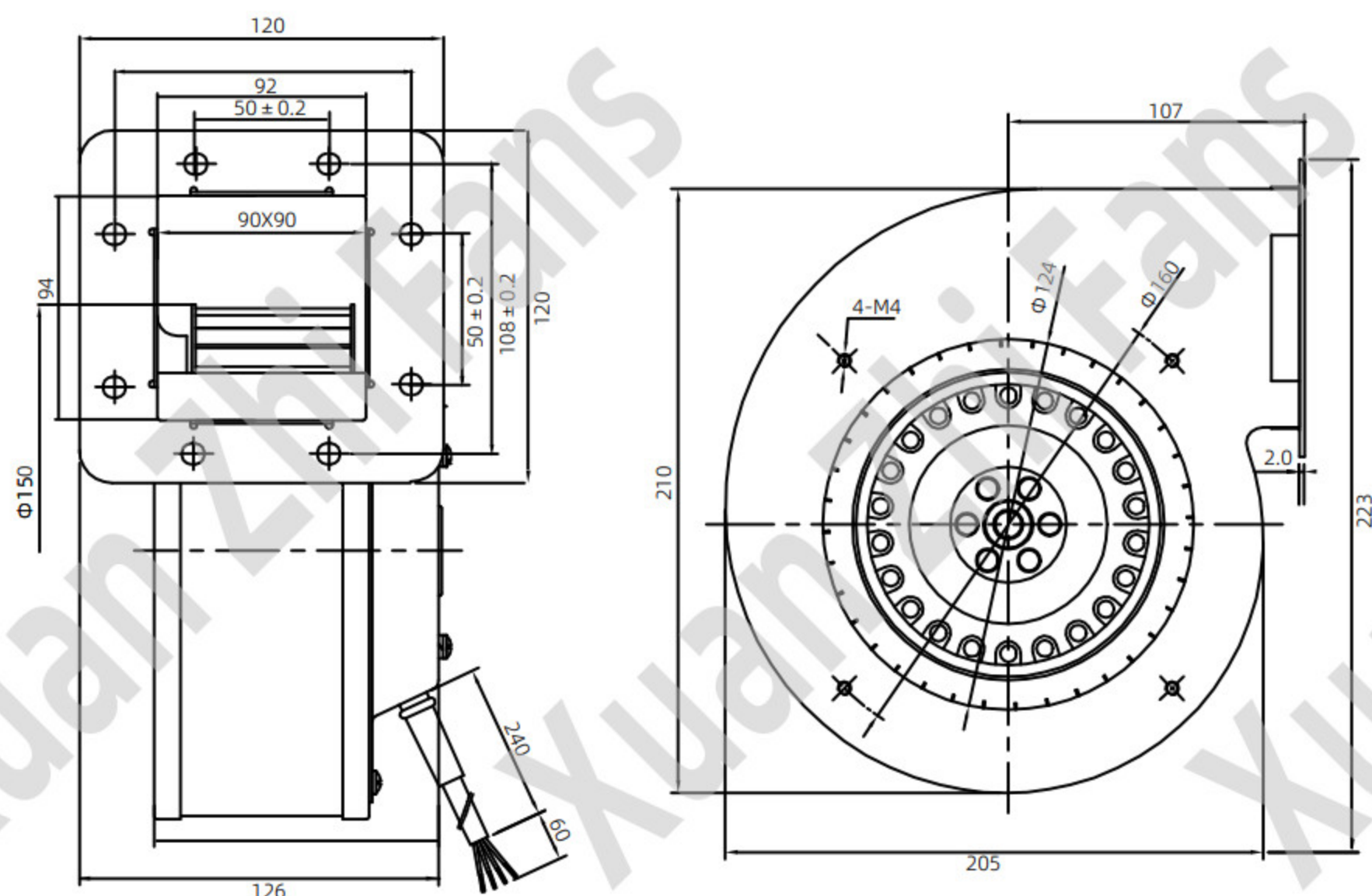
尺寸图Dimension Drawing (Unit : mm)
