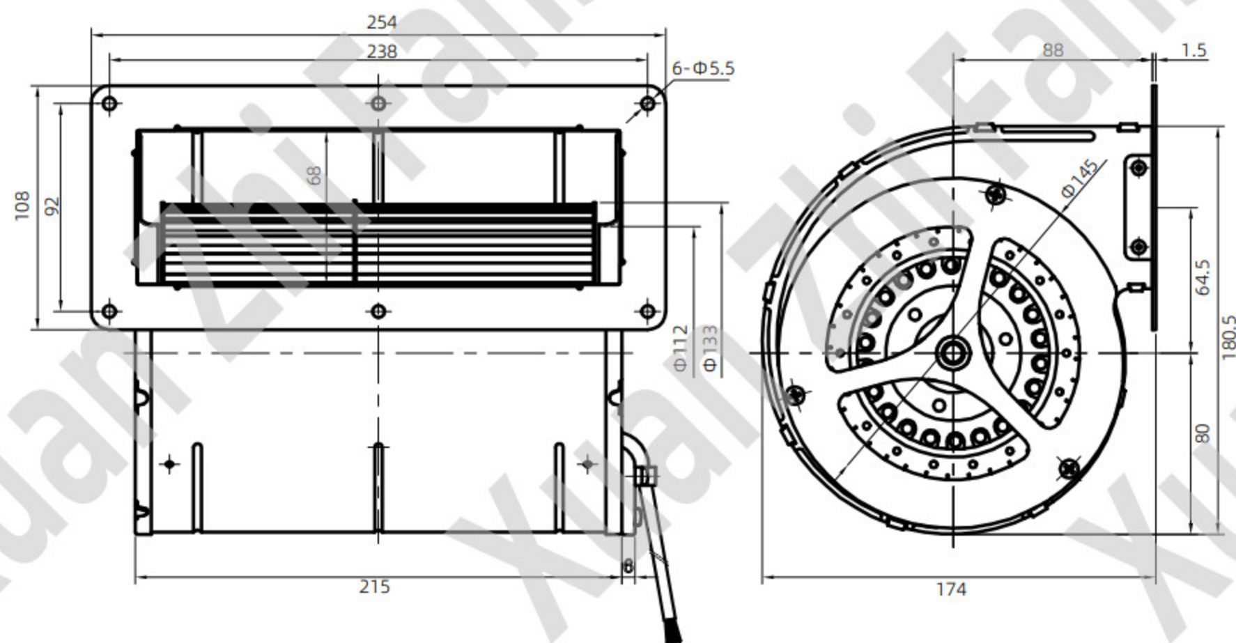
尺寸图Dimension Drawing (Unit : mm)
