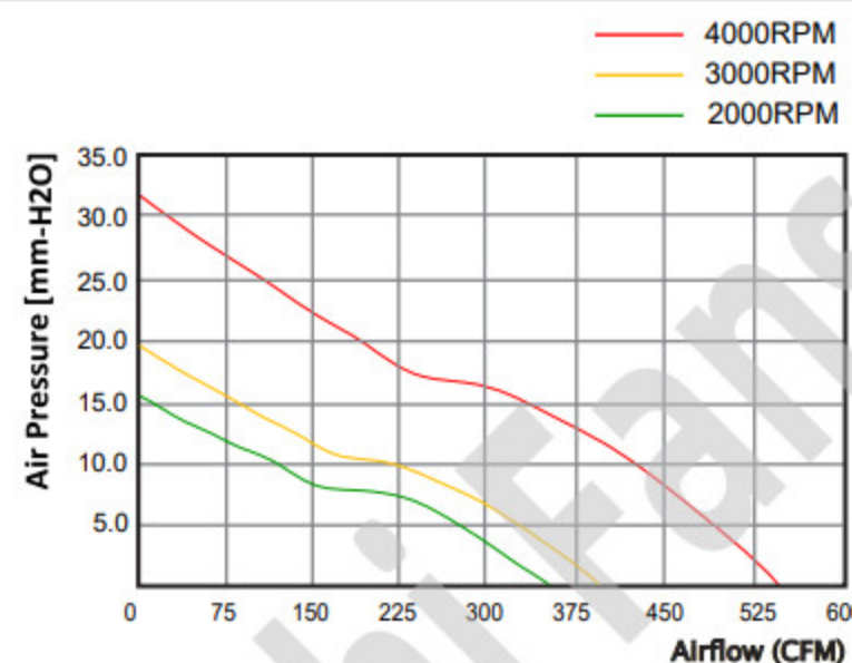
P-Q 曲线图/P-Q Curve Chart
