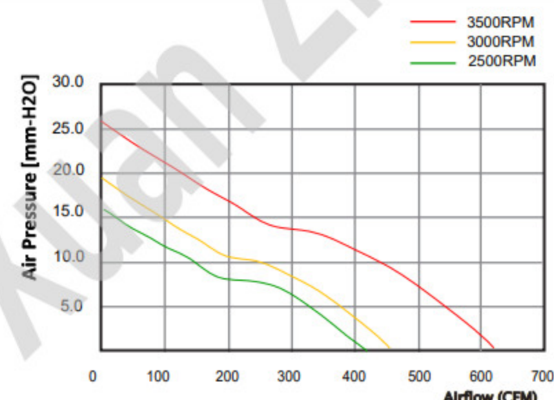
P-Q 曲线图/P-Q Curve Chart
