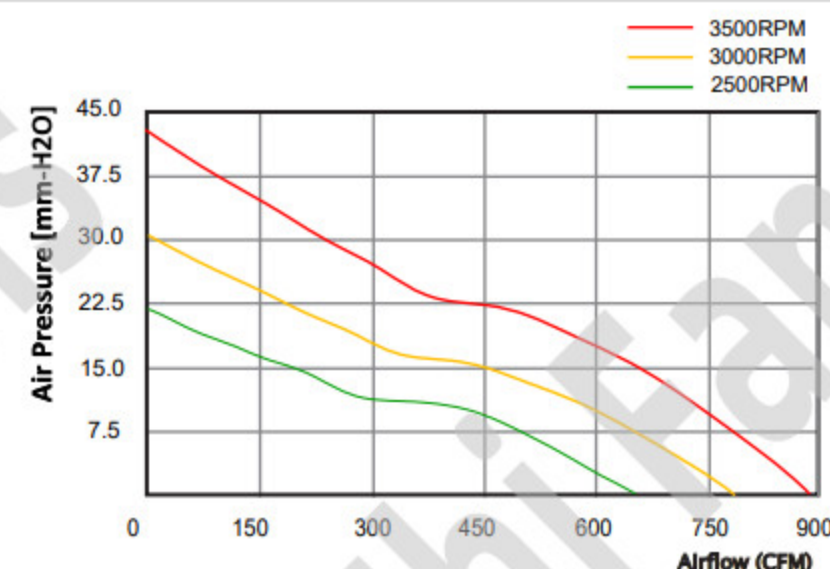
P-Q 曲线图/P-Q Curve Chart
